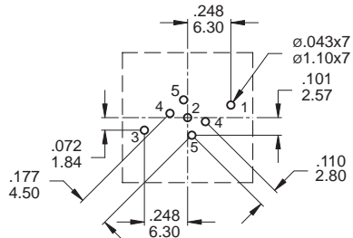
KS9B/C CAP Type TOP VIEW
