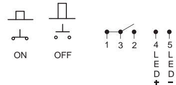
CIRCUIT
