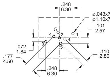
KS9B/C CAP Type TOP VIEW
