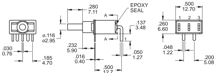
SECTION A-A TERM. NOS. FOR REFERENCE ONLY
