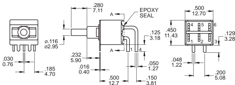
SECTION A-A TERM. NOS. FOR REFERENCE ONLY
