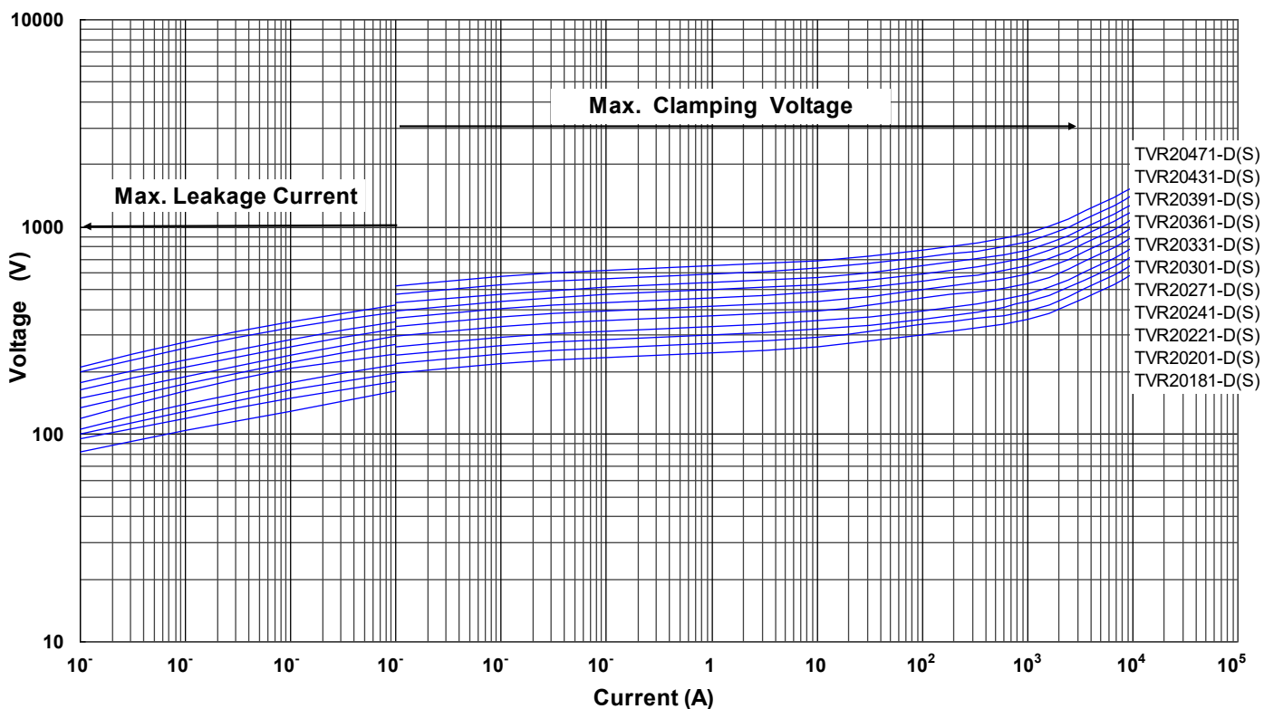
Max. Leakage Current and Max. Clamping Voltage Curves (TVR20481-D(S) to TVR20471-D(S))
