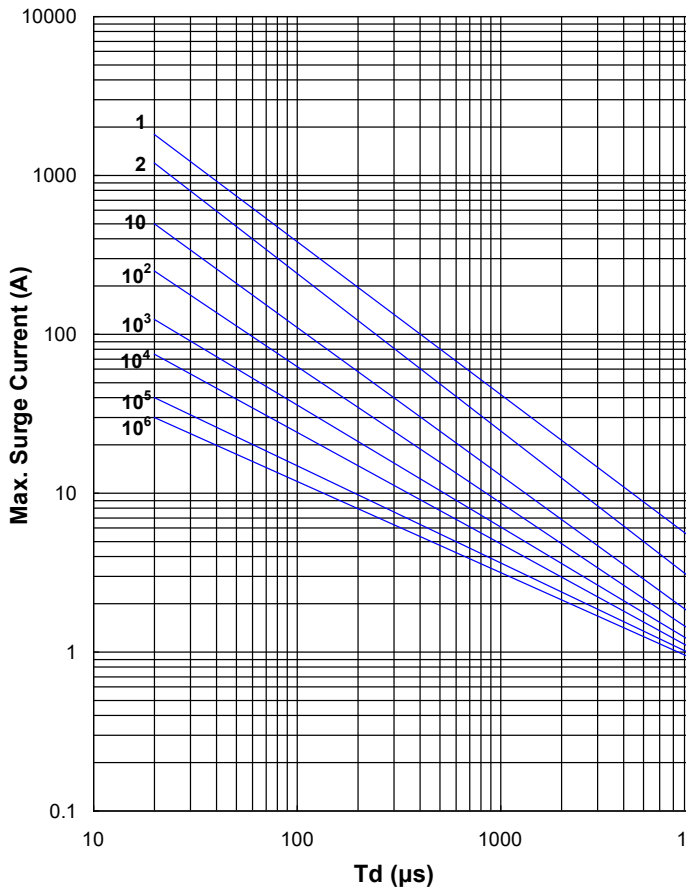
TVR07181-D to TVR07471-D
