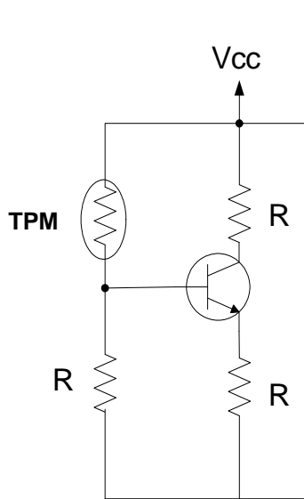
Fig 1. Overheat Protection
